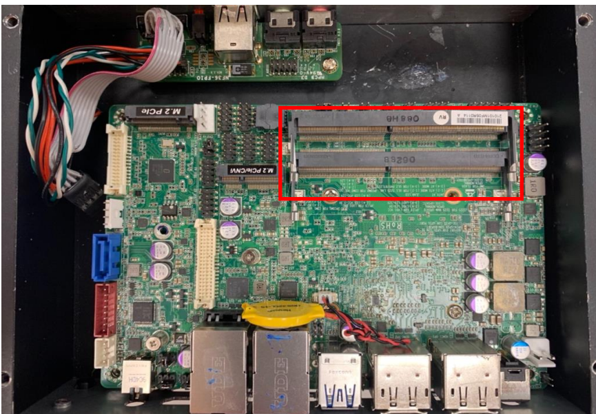
1. Locate the SO-DIMM slot on the board.
