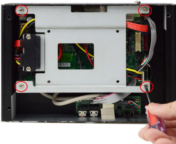
6. Remove the marked screws to disassemble the HDD tray from the system.
