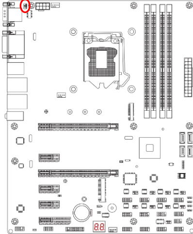
JP1 → COM1 Port
