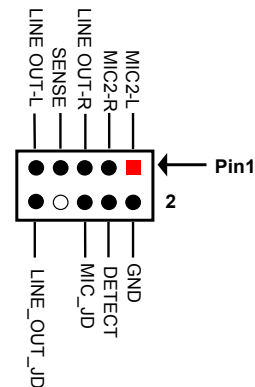
Line-Out, MIC Header
